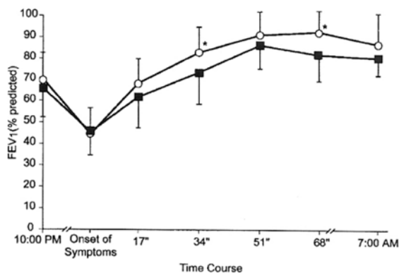
Figure 6. Forced expiratory volume in 1 second (FEV 1 ) in 8 subjects with asthma during a nocturnal asthma attack. Subjects were treated with doubling doses at 15-minute intervals with albuterol metered-dose inhaler (MDI) (○) or epinephrine MDI (Primatene Mist, Wyeth Pharmaceuticals, Madison, NJ) (■) in a randomized, crossover manner. FEV 1 was significantly higher after albuterol at 34 and 68 minutes but the differences were not clinically relevant. Reproduced with permission from Annals of Allergy, Asthma, and Immunology . 28
